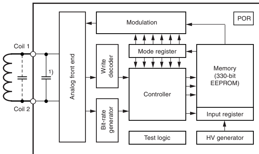
Figure 3-1. Block Diagram
