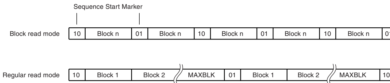
Figure 6-2. ATA5567 Sequence Start Marker in Extended Mode
