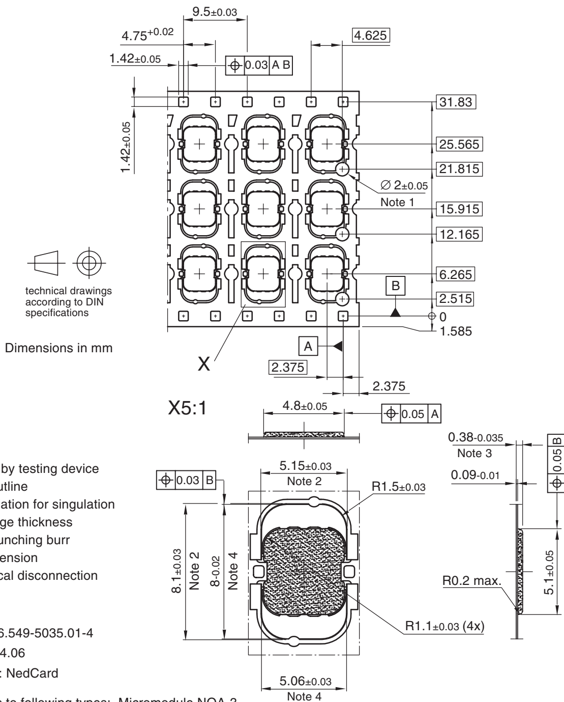
Figure 10-5. NOA3 Micromodule
